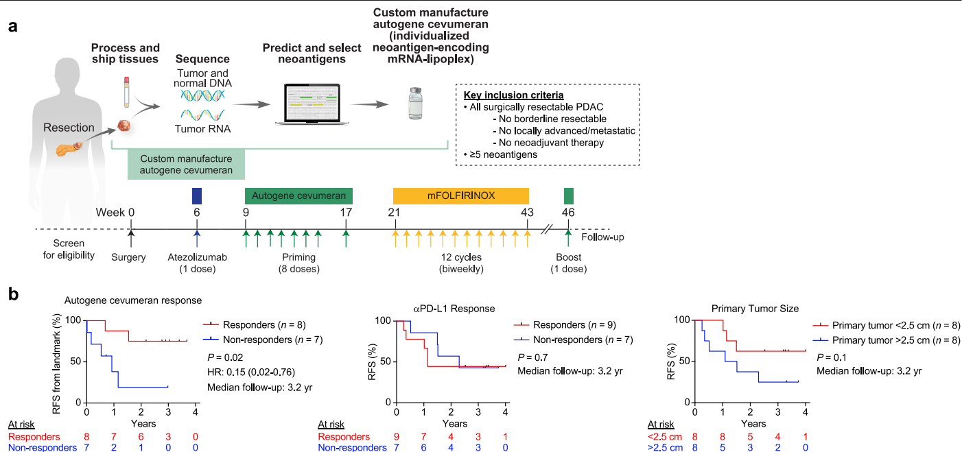
Extended Data Fig. 1 | Autogene cevumiran but not atezolizumab response or tumor size correlates with RFS at 3-year follow-up. a , Trial schematic as previously reported 1 . Reproduced under CC BY 4.0: https://creativecommons.org/licenses/by/4.0/ . b , Recurrence-free survival (RFS) from landmark time (last vaccine priming dose) stratified by autogene cevumiran (vaccine)
